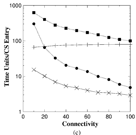
—+— RL, High Load Delay between CS release & next request = 1 time unit. .....■..... RR, High Load —x— RL, Low Load Delay between CS release & next request = 1000 time units. .....●..... RR, Low Load
