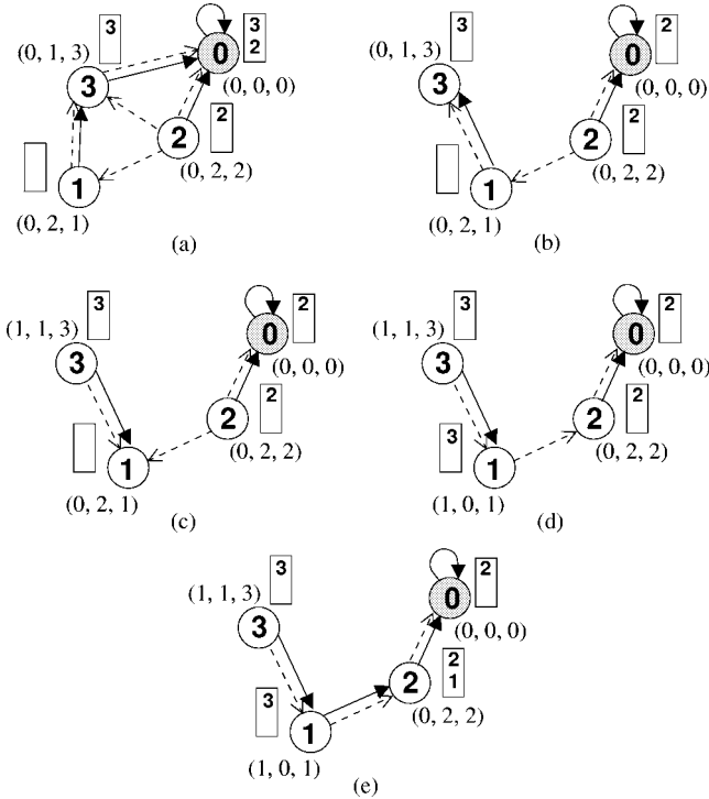
Figure 8. Operation of reverse link mutual exclusion algorithm on dynamic network.
