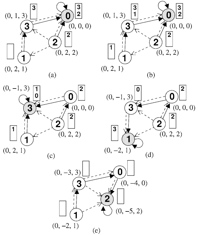
Figure 7. Operation of reverse link mutual exclusion algorithm on static network.
