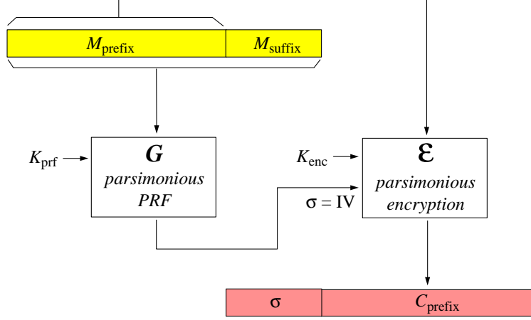
Figure 2: A general description of VIL mode. The ciphertext is \sigma || C_{\text{prefix}} . The value \sigma is the output of the PRF G , the IV to the encryption scheme, and the first n bits of ciphertext.
