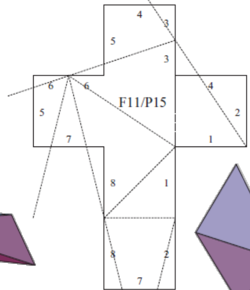
hexahedron
