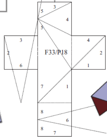
octahedron
