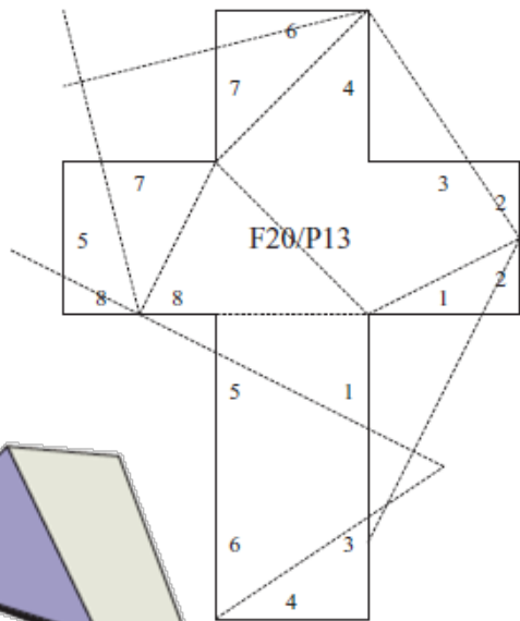
pentahedron
