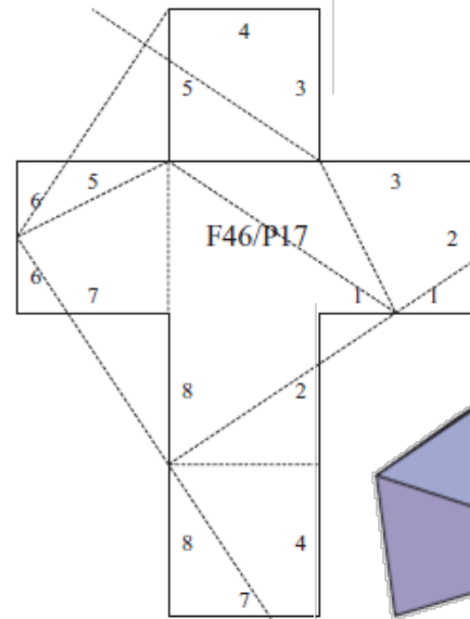
hexahedron
