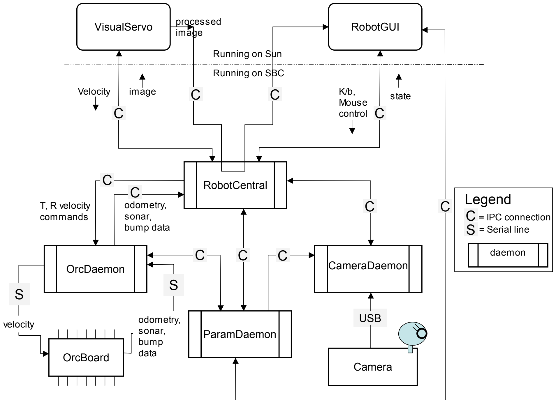
Carmen block diagram
