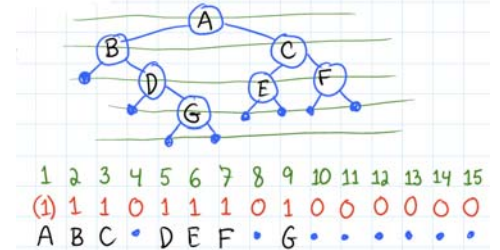
SUCCINCT
