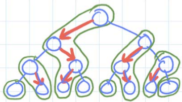
DYNAMIC OPTIMALITY
