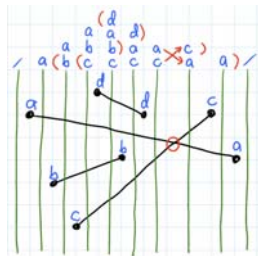
GEOMETRY
