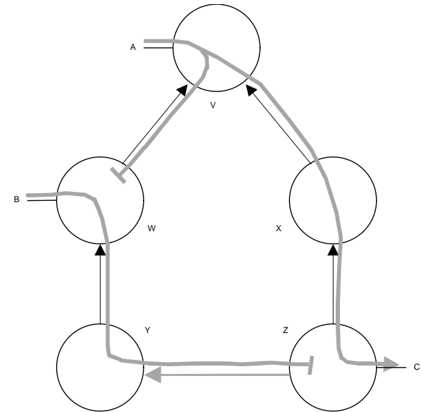
Figure 9: Broadcast deadlock
