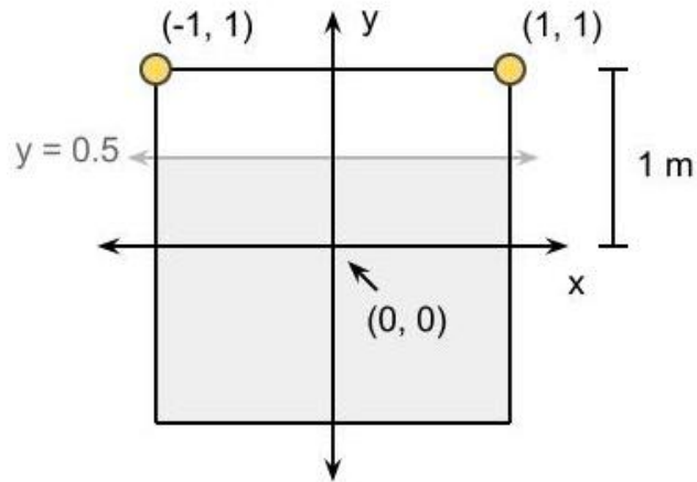
Figure 2: Locations of the two light sources and shaded region for the unknown robot location.
